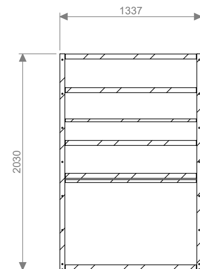
A-A SECTION HATCHED AREA IS THE BASE SUPPORT GROUND REST
